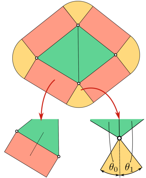
Fig. 3. Two different types of Voronoi Region. The orange zone is defined as the rectangular Voronoi region, and the yellow zone is defined as the sectoral Voronoi region.
