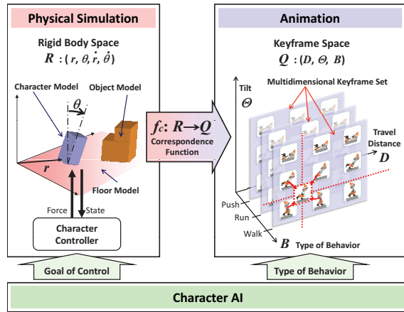
Figure 1: Overview of the proposed method
